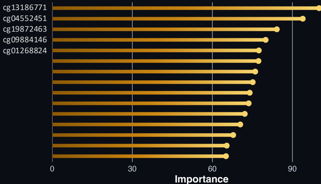
Random Forest Variable Importance
